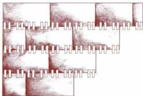
Correct: "T"-joints for all types of slabs
